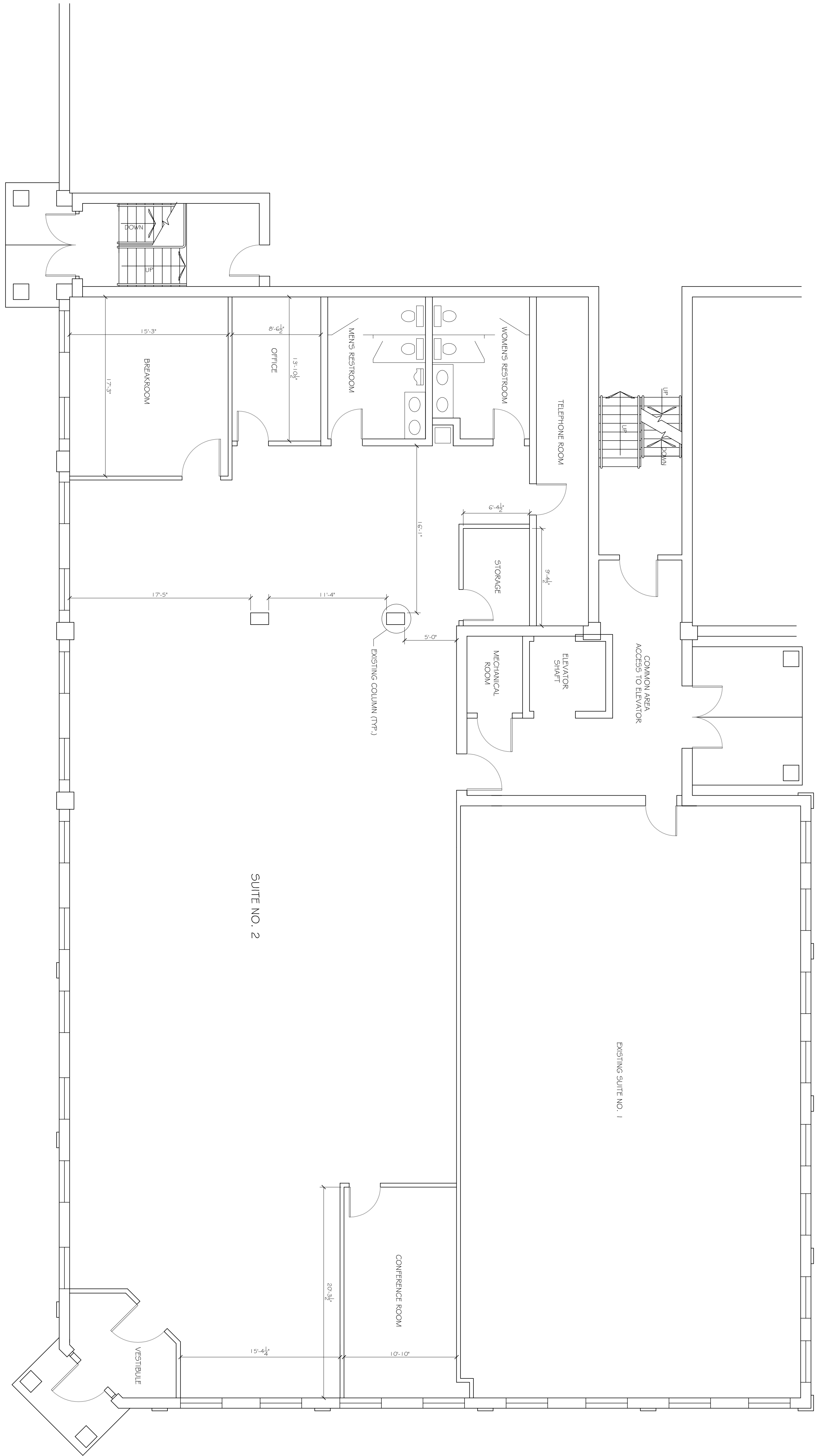
FIRST FLOOR PLAN SUITE NO. 2 1425 MT READ BLVD. SCALE: 3/16"=1'-0"
