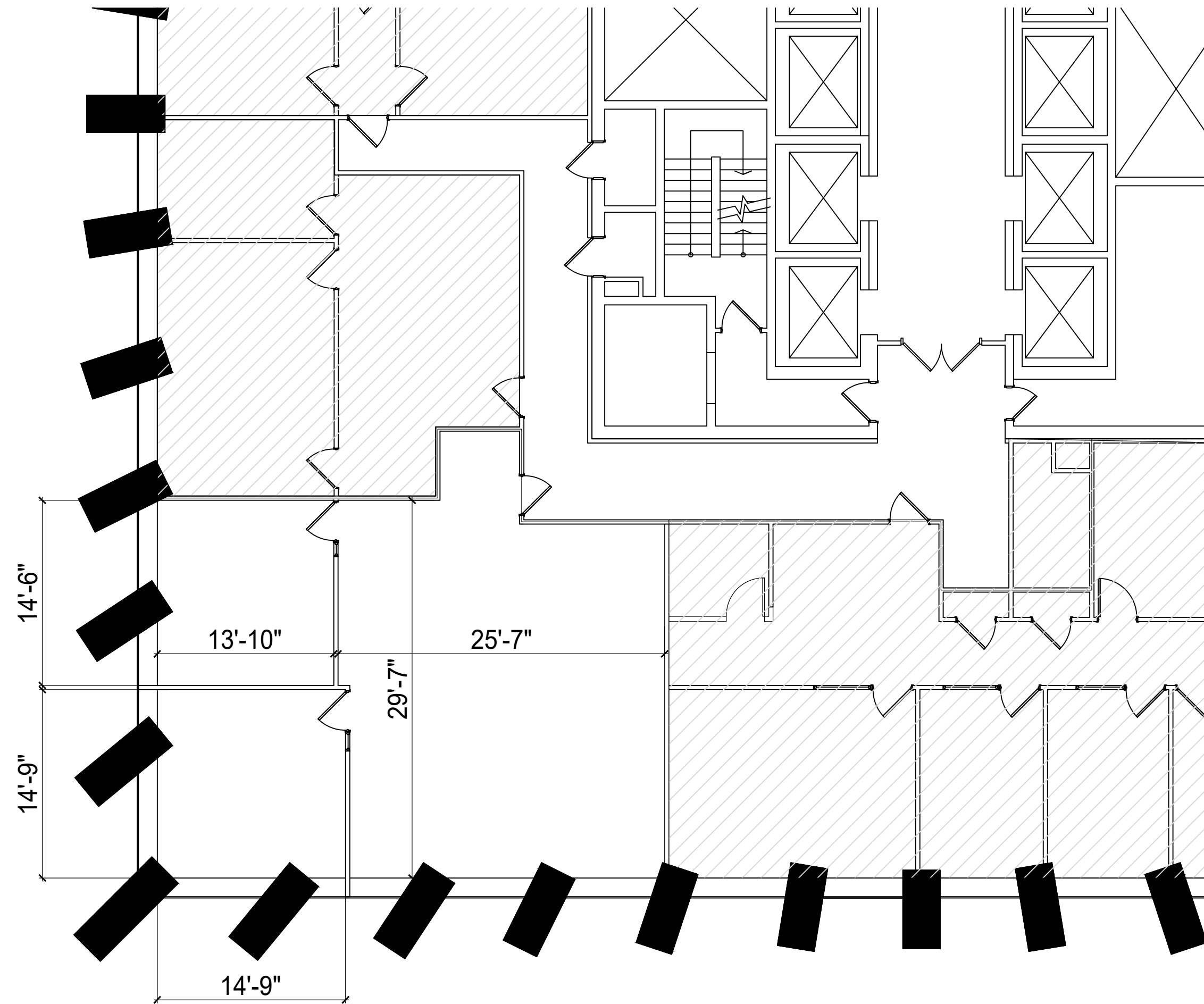
1 10TH FLOOR PLAN SCALE: 1/8" = 1'-0"
